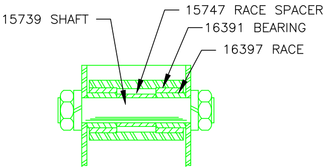
DETAIL "D"
